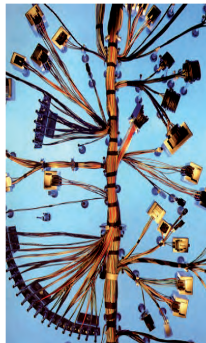
Figure 2: Typical CAN wiring harness (Photo: Bosch)
