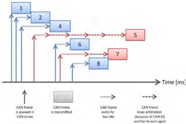
Figure 2: Timing diagram of CAN network with focus on arbitration delays (in red) (Photo: Syntavision)
