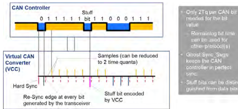
Figure 8: Reduced CAN Protocol principle (Source: Kvaser)
