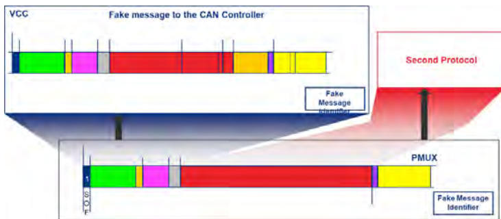
Figure 17: Integrated protocol multiplexing fake frame embedding reception (Source: Kvaser)
